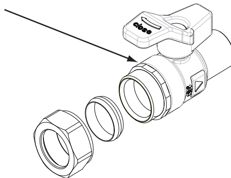
Figure 17 - Exploded View of Isolating valve
