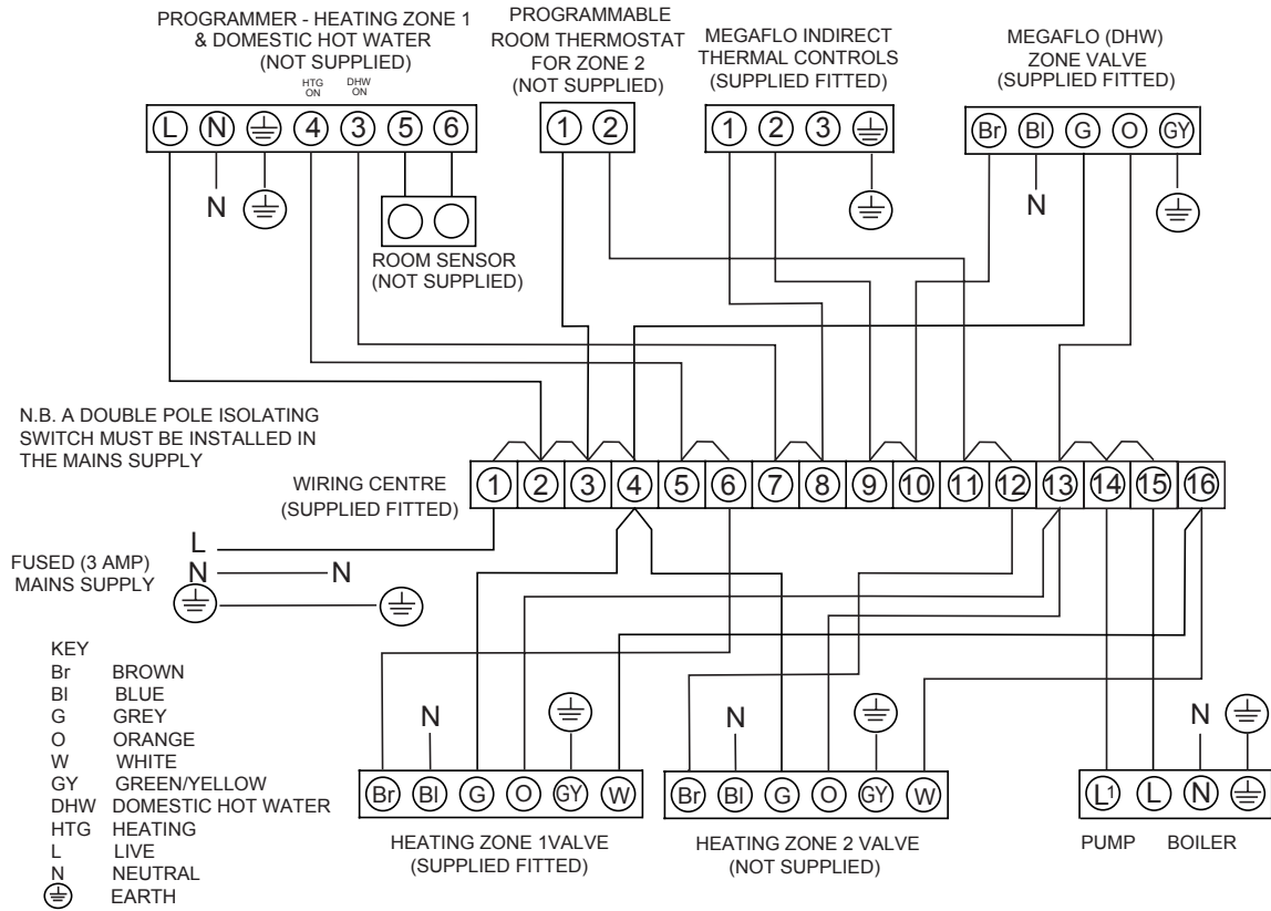
Figure 13 - Schematic Wiring Diagram - Indirect Circuit
