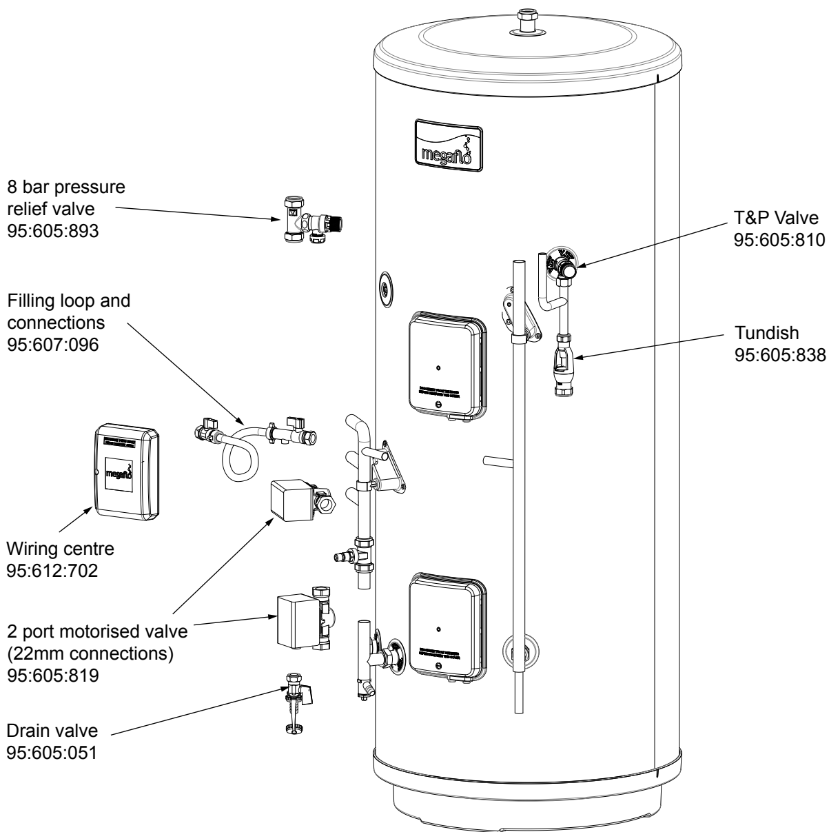
Figure 19: SystemReady Exploded View
