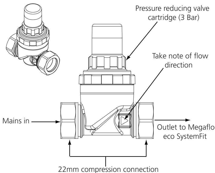
Figure 3 - 3 Bar Pressure Reducing Valve
