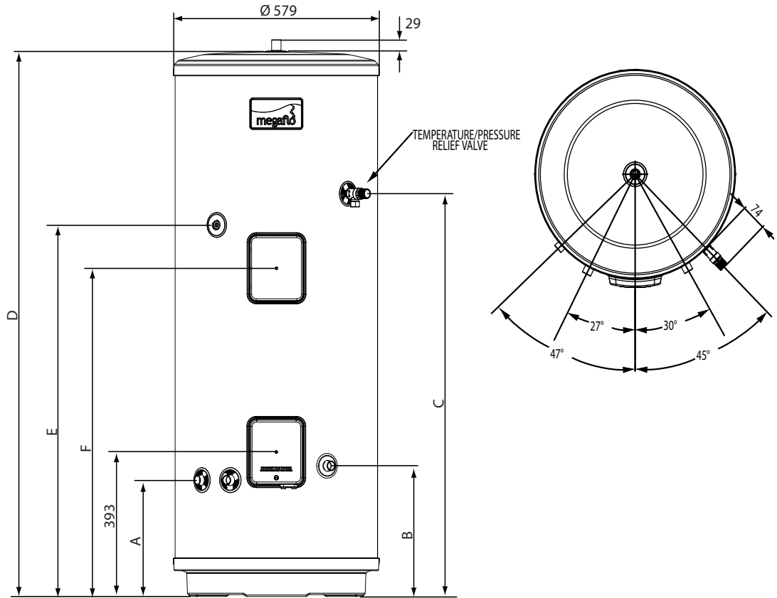
Figure 2 - Megaflo eco SystemReady Indirect
